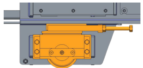
Height-adjustable rollers on the press ram
